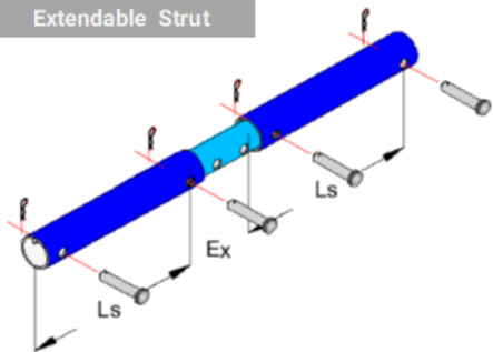
Extendable Strut
