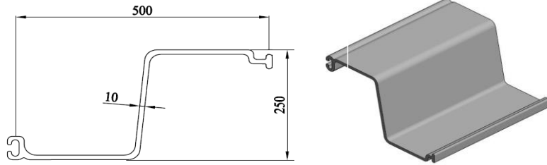
ESC VINYL SHEET PILE PROFILE ESC-VU80
