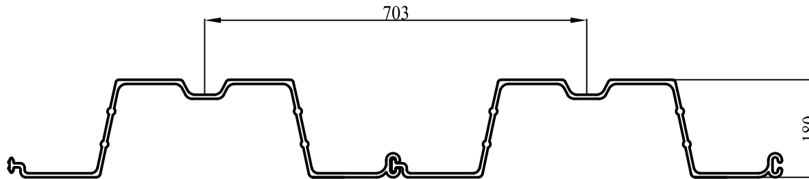
VINYL SHEET PILE COMBI WALL
