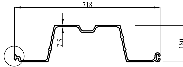
ESC VU703-7.5 VINYL SHEET PILE PROFILE
