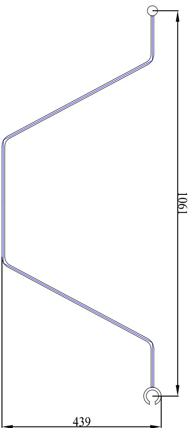
SHEET PILE PROFILE
