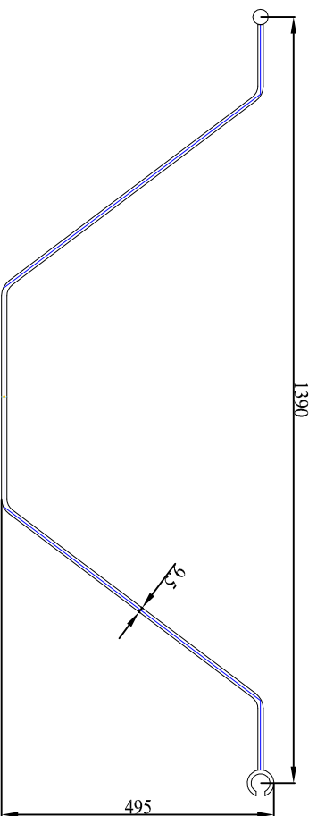
SHEET PILE PROFILE
